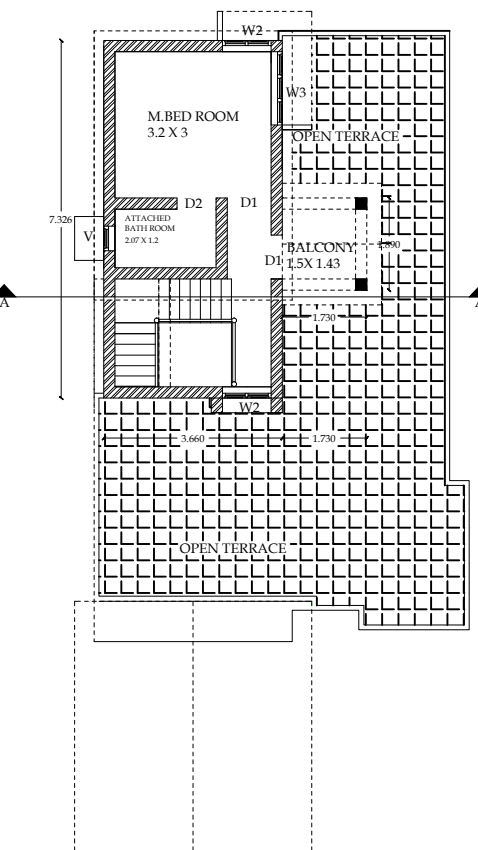
FIRST FLOOR PLAN AREA-30.08 sq m
