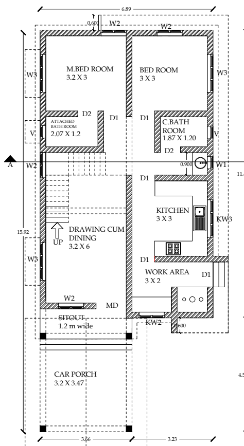
GROUND FLOOR PLAN AREA-95.62 sq m
